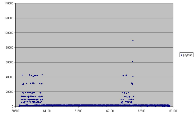
Session Payload 8 x 100 Sessions x 2 Servers Load Balanced
